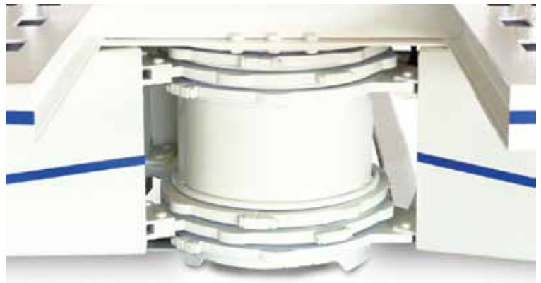
Three towers pivot from the large drum which also stores the electric over hydraulic pump.
