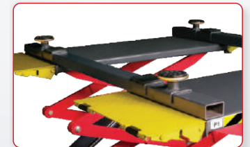
Optional Support Bars&Kits. Recommended for heavier vehicles with narrow frames.
