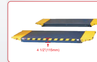
Low profile design, the closed height is only 4 1/2"(115mm).
