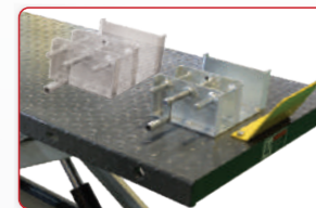
Front wheel vise Front wheel vise with an adjustable positioning distance of 16 1/8" (410mm).
